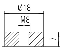
Terminal F-M8
