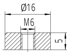
Terminal F-M6
