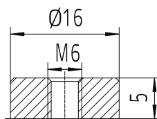
Terminal F-M6
