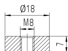
Terminal F-M8
