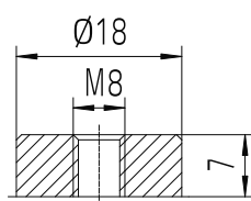
Terminal F-M8
