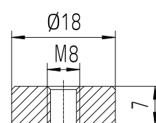
Terminal F-M8
