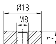
Terminal F-M8
